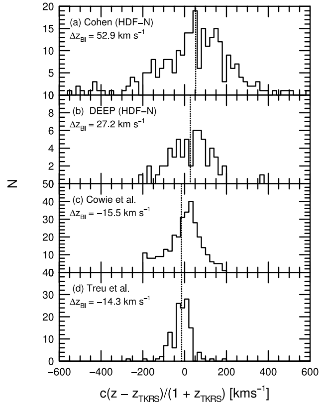
FIG. 13.— Histogram showing the redshift differences between galaxies with secure measurements in the TKRS vs. four other extensive samples in the GOODS-N region. Each panel shows the bi-weight location ( dotted line ) and its value (Beers et al. 1990). (a) Redshift differences for galaxies with secure measurements from LRIS in Cohen et al. (2000) and Cohen (2001). (b) Redshift differences between TKRS and secure measurements of Phillips et al. (1997) and Lowenthal et al. (1997), also using LRIS. (c) Redshift differences with the Cowie et al. (2004) sample of galaxies, which used similar instrumental setup and integration times as the TKRS. (d) Redshift differences with the Treu et al. (2004) sample of galaxies observed with DEIMOS but using higher resolution and longer integration times than this work.
